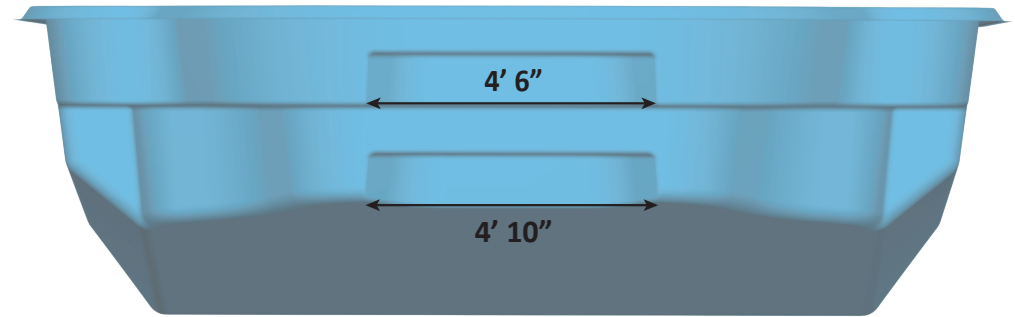
Step Ends A & B Widths
