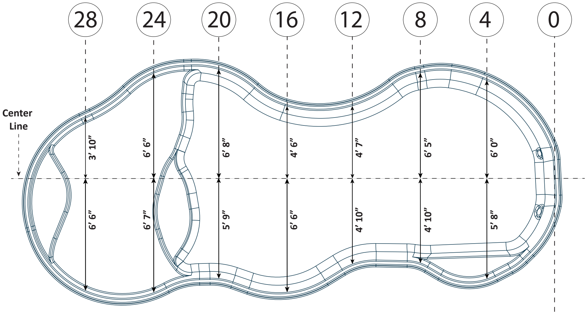
Distance to Curves from Center Line
