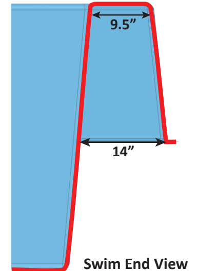
Cross Section 2
